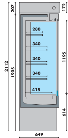
MURAL COM ESTORES ELÉTRICOS ELECTRIC SHUTTER MULTIDECK
